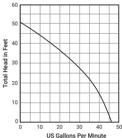
PERFORMANCE CURVE
