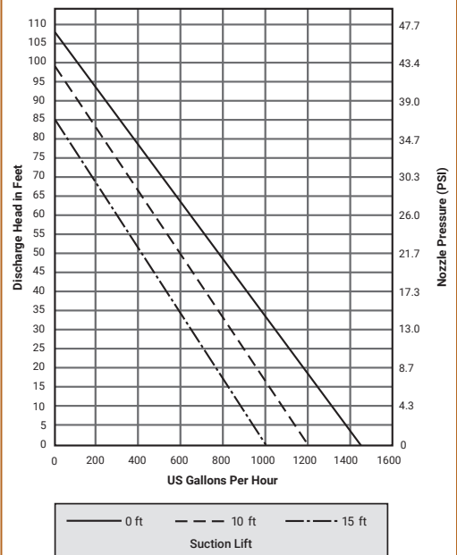
PERFORMANCE CURVE
