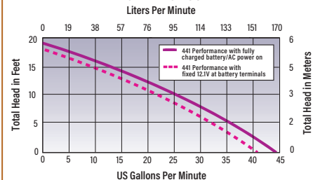
PERFORMANCE CURVE
