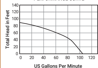
PERFORMANCE CURVE
