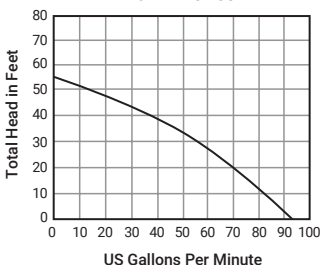
PERFORMANCE CURVE
