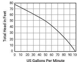
PERFORMANCE CURVE
