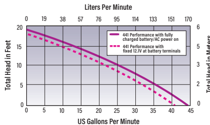
PERFORMANCE CURVE
