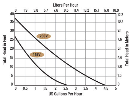
PERFORMANCE CURVE
